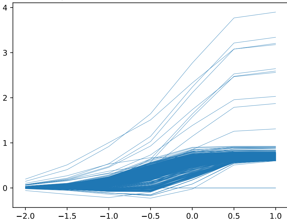
Dynamic Ricci Curvature for Geodesic 0.0
